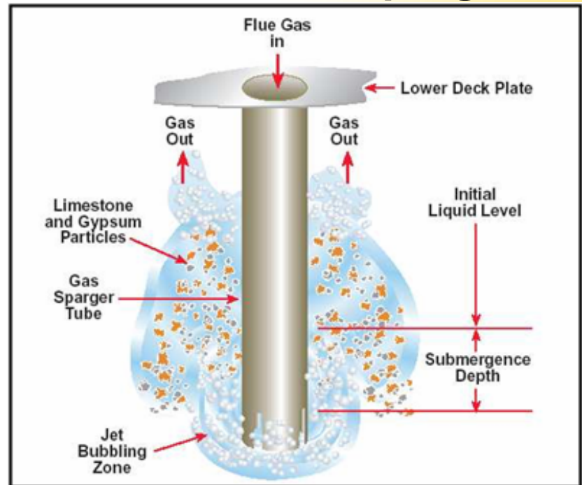
Individual Sparger
