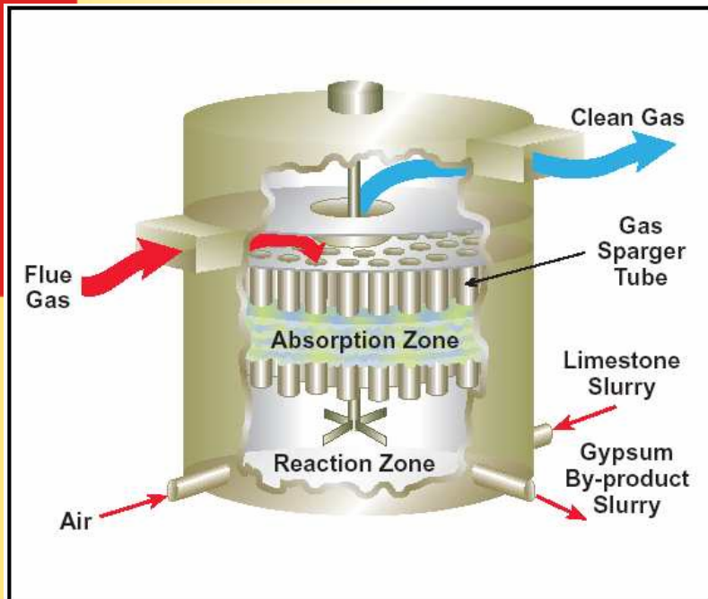
Reactor
